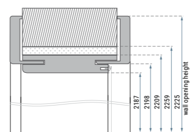
Dimensions of door frame for PN22 door.
