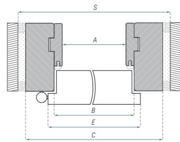
Dimensions of FIRE fixed door frame [mm]:
