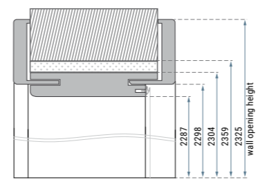
Dimensions of door frame for PN23 door.
