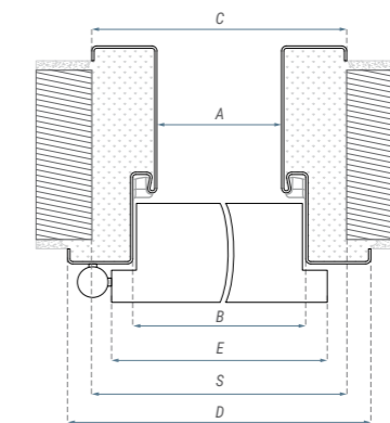
Dimensions of BORD fixed door frame [mm]:
