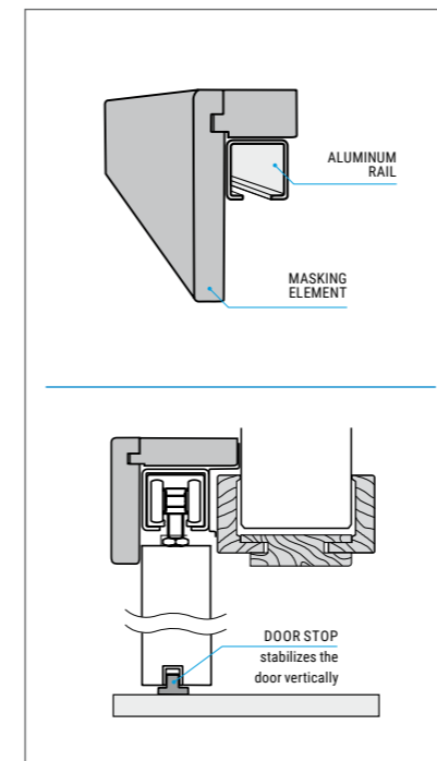
VERTICAL CROSS-SECTION OF THE SLIDING SYSTEM
