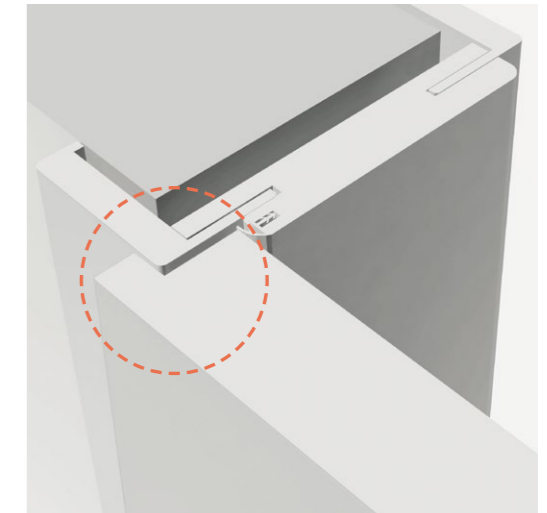
REBATED DOOR
