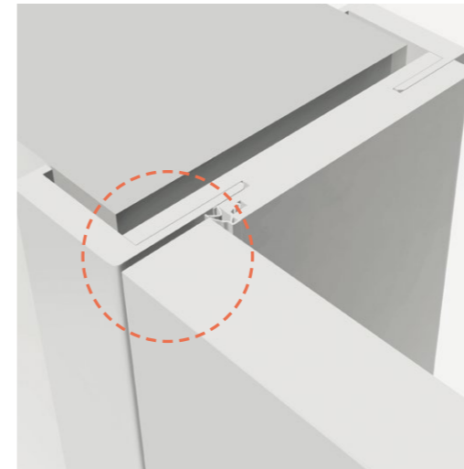
NON-REBATED DOOR
