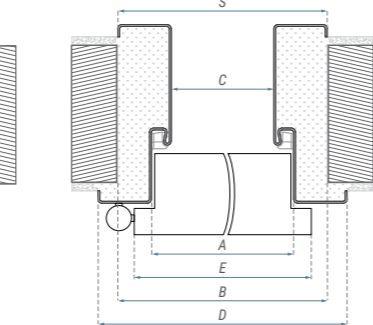
Dimensions of FIRE wooden door frame [mm]:
