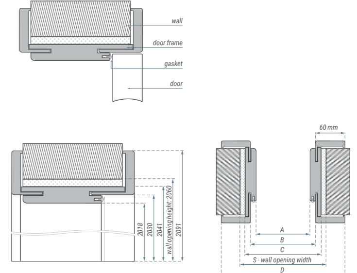
▲ ADJUSTABLE NON-REBATED DOOR FRAME
