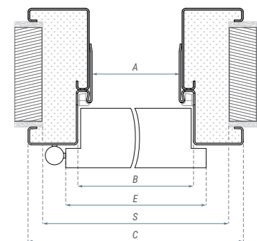
Dimensions of GUARD Adjustable door frame [mm]:
