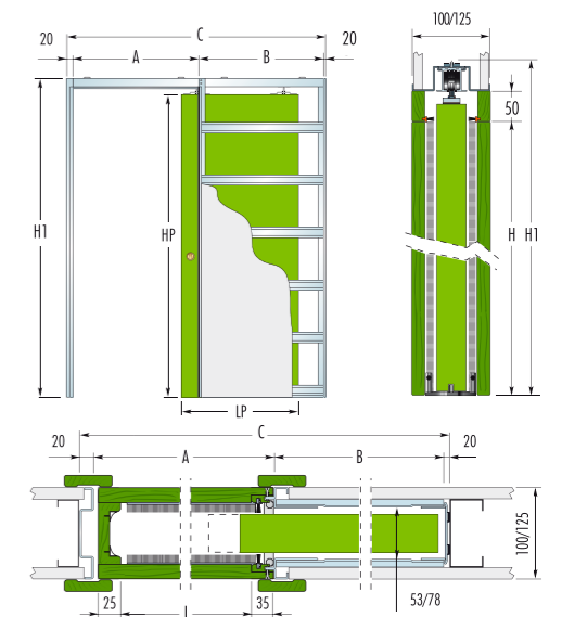
SINGLE POCKET DIMENSION TABLE
